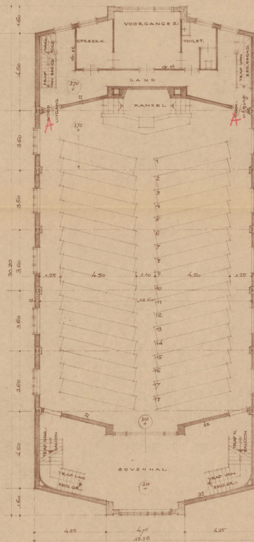
ZAALVERDIEPING.
